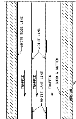
MARKING PLACEMENT DETAIL
